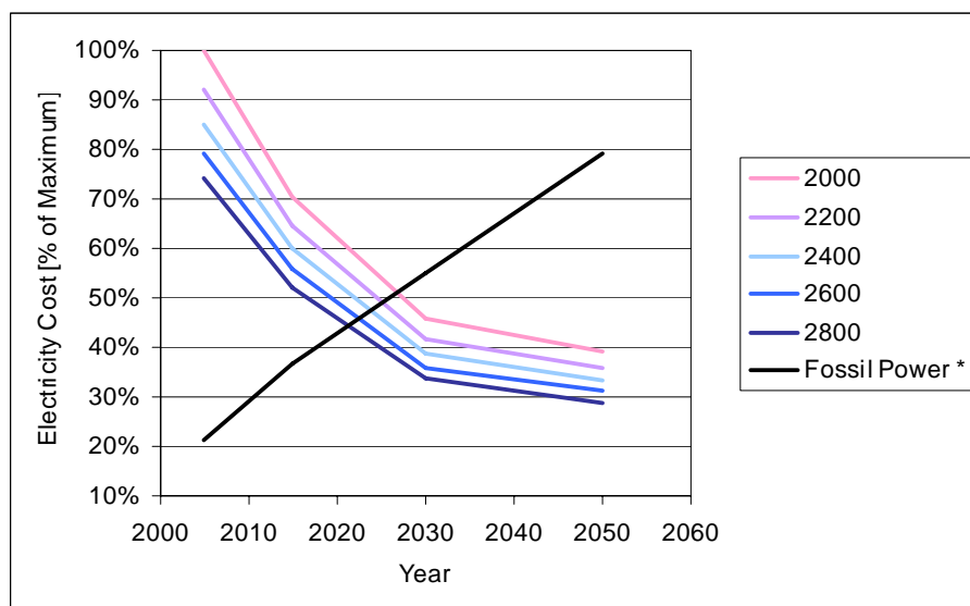
Fig. 8. Electricity cost in % of the maximum starting value in 2005 as function of time and direct normal irradiation (DNI in kWh/m²/y) for CSP reference plants with a solar multiple SM4 compared to the cost of power generation from fossil fuels (including carbon costs) according to [9]*
