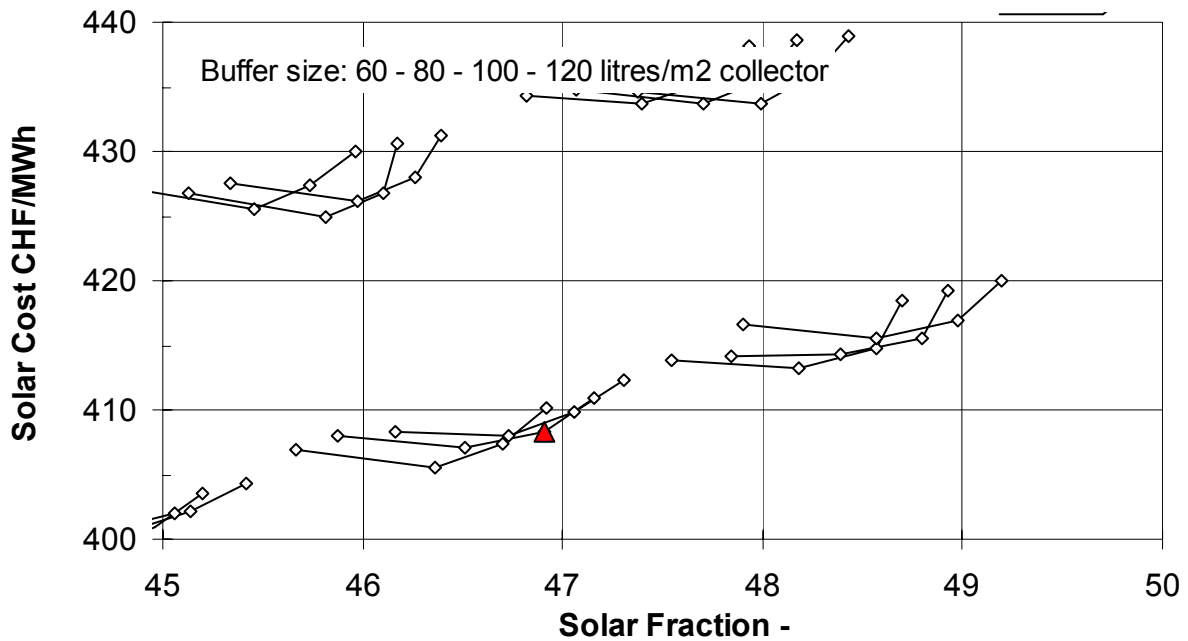
Figure 6.4: Zoom in the buffer store volume curves.
