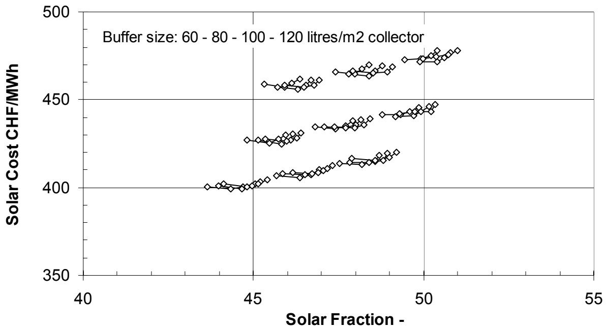
Figure 6.3: Buffer store volume curves in the diagram “solar cost” – “solar fraction” for the variant “Hochhaus + Kurzhaus + Langhaus”.
